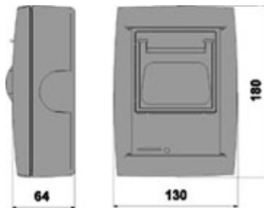
OBTPRB - dimensions in mm
